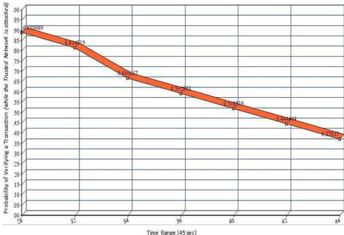
Figure 5.1.1 Man-in-the-Middle Attack Evaluation Results
