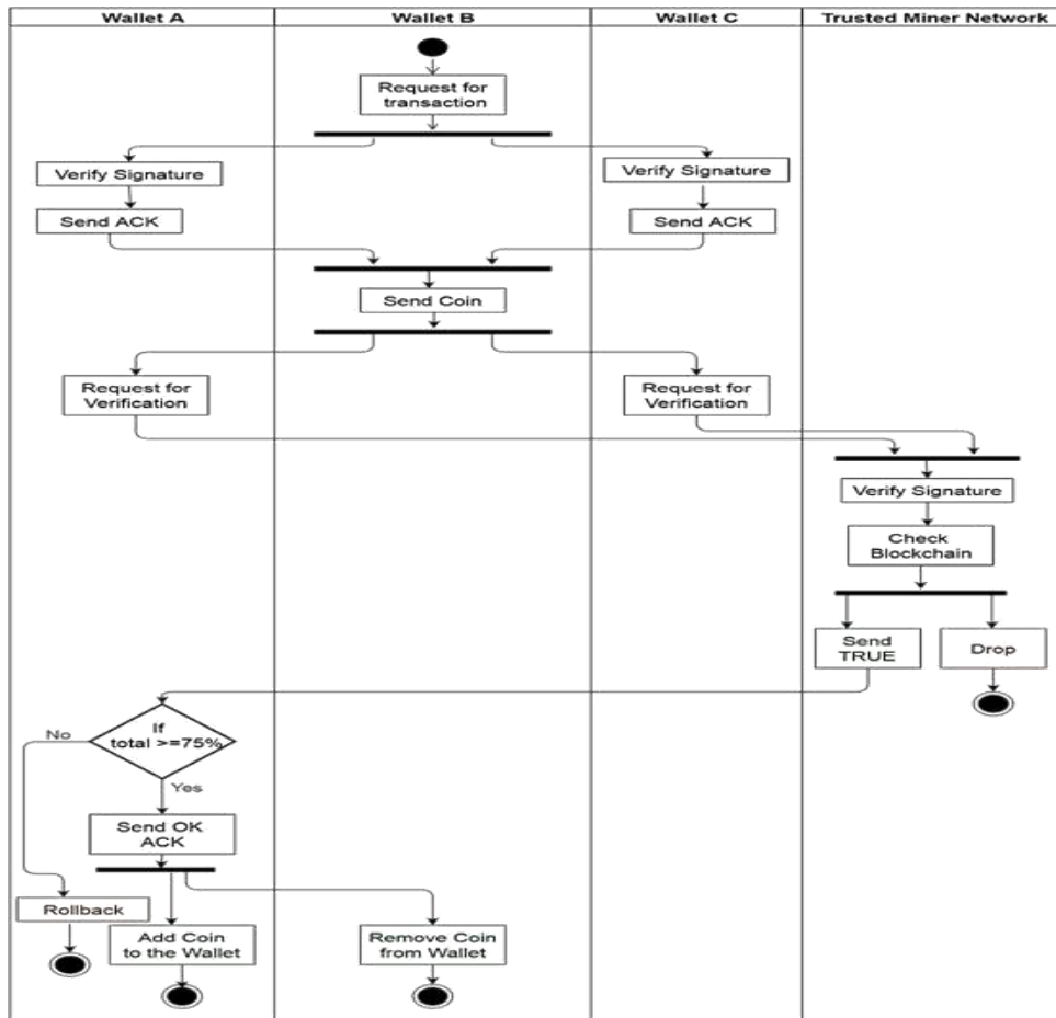
Figure 5.2.1 Double Spending Evaluation
