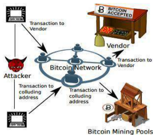
Figure 2.3.1 A Double Spending Attack against Fast Payments in Bitcoin (G.Karame, et al., 2015)
