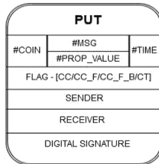
Figure 3.3.2 Protocol Design: ‘PUT Protocol
