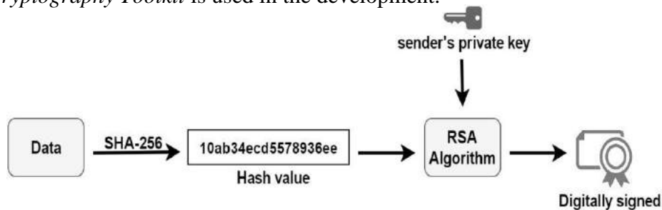
Figure 4.3.1 Asymmetric Digital Signature Generation
