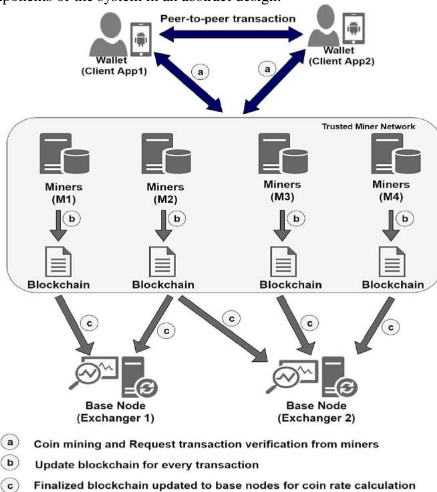
Figure A. 1 Social Currency Payment Platform Architecture
