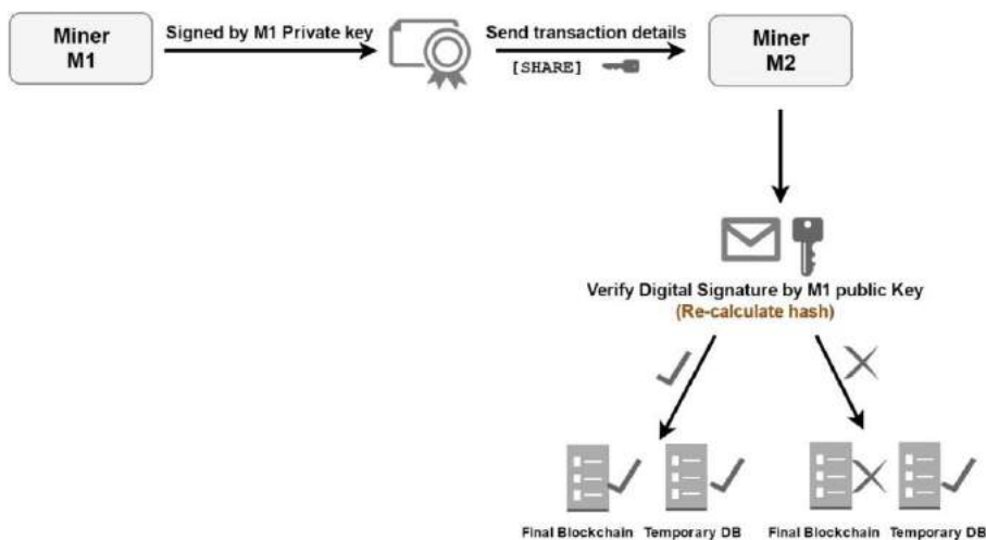
Figure 3.4.3 Scenario B: Miner-Miner Transaction Verification Model
