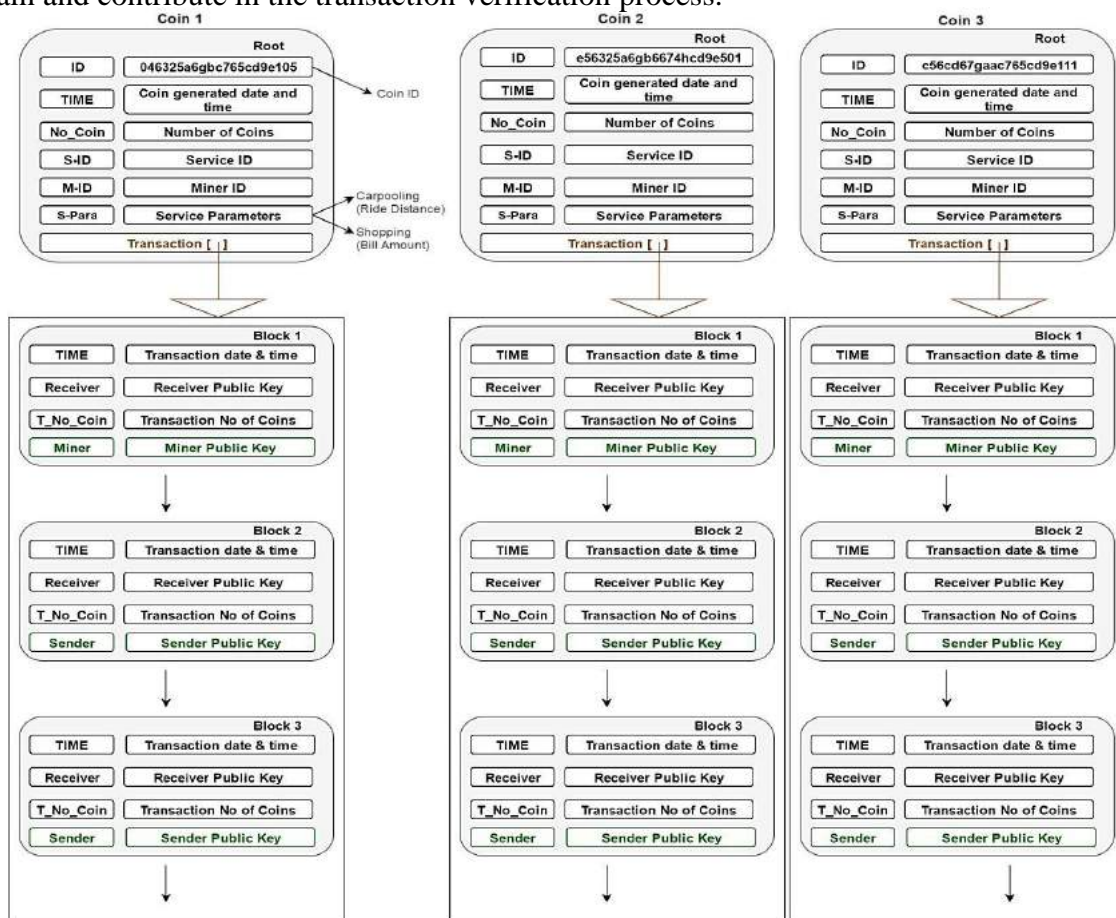
Figure B. 1 Coin Wise Blockchain Design
