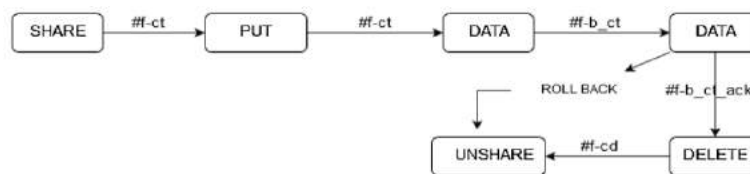
Figure 4.2.1 Miner to App and Miner to Miner Protocol Implementation
